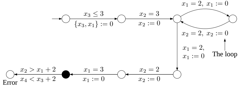
Fig. 18: Timed automaton \mathcal{A} which makes the forward analysis fail
