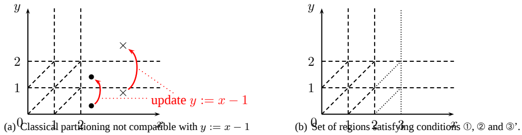
Fig. 12: Partitioning for updates of the form y := x - 1
