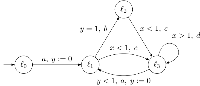
Fig. 4: An example of timed automaton
