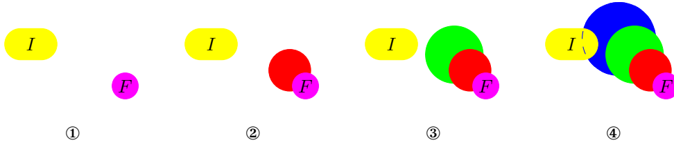
Fig. 14: Backward analysis: step by step, predecessors of final configurations are computed
