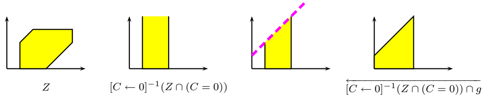
Fig. 16: Example of backward computation for timed automata (Pre operator)
