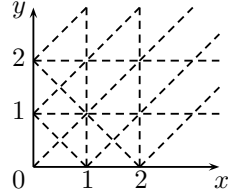
Fig. 8: Region partitioning for additive clock constraints (two clocks)
