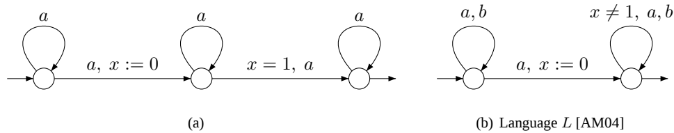
Fig. 6: Two non-complementable timed automata
