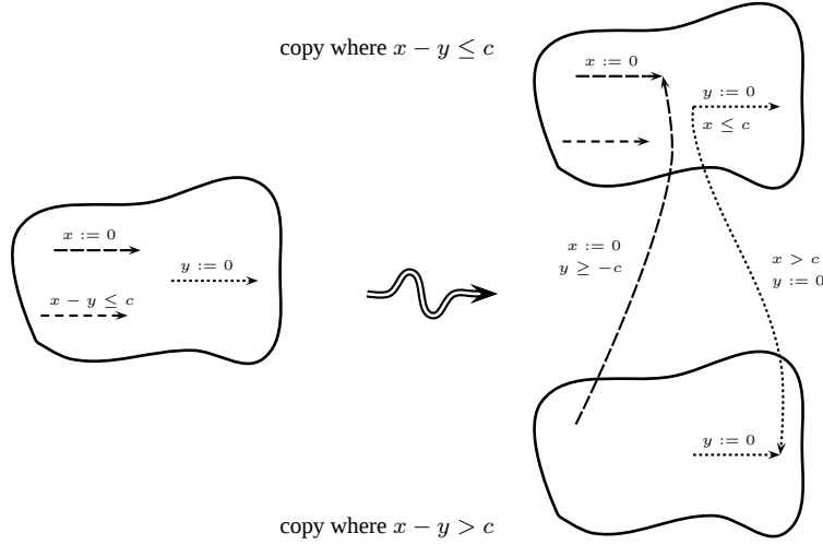
Fig. 7: Erasing diagonal constraint x - y \leq c
