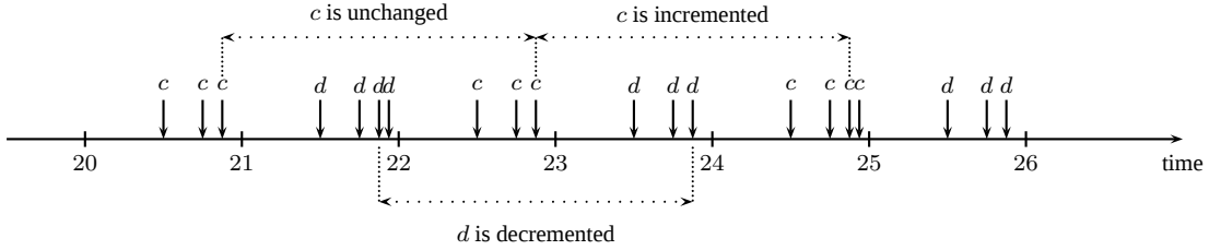
Fig. 10: Encoding of a two counter machine
