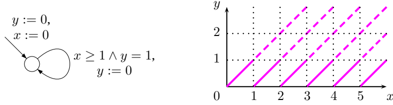
Fig. 17: Forward computation does not always terminate...
