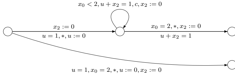
Fig. 11: Incrementation of counter c
