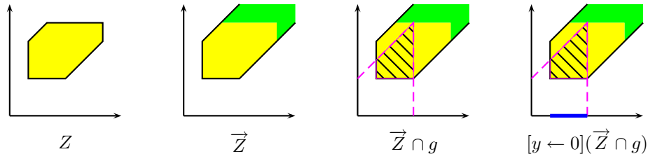
Fig. 15: Example of forward computation for timed automata (Post operator)
