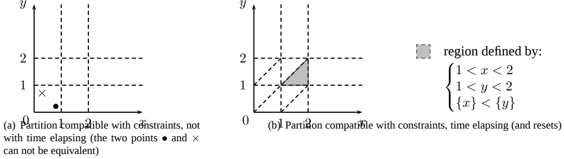
Fig. 2: Diagonal-free region partitioning for two clocks and maximal constant 2
