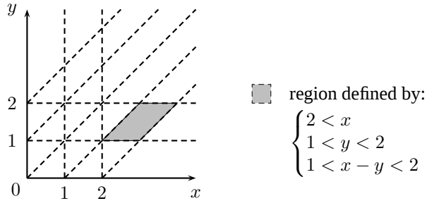
Fig. 3: Set of regions for 2-bounded general constraints with two clocks
