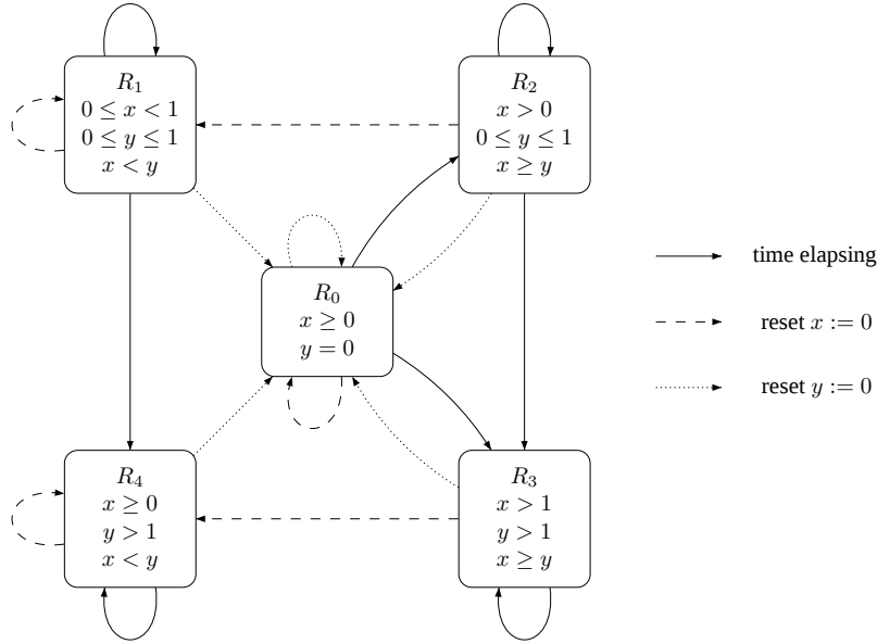
Fig. 1: A simple example of region graph
